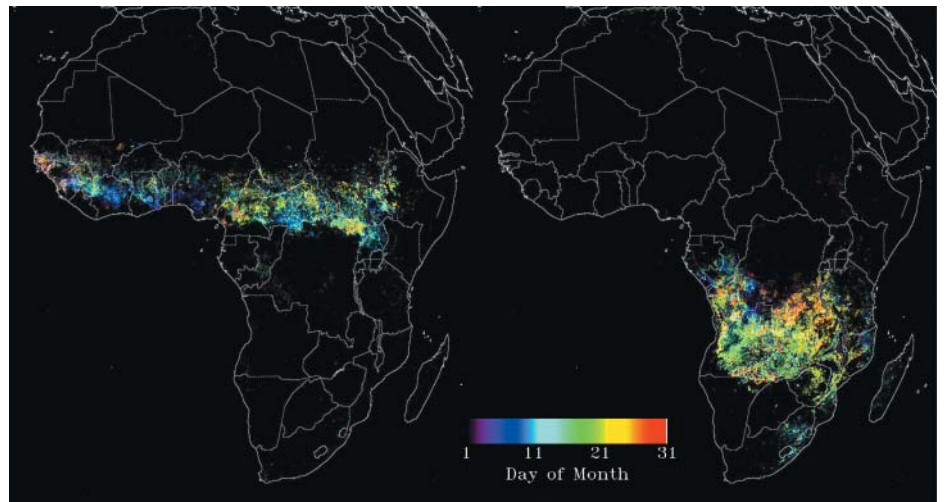
Fig. 2. SEVIRI-derived maps of active fire detections for (left) February and (right) August 2004.
