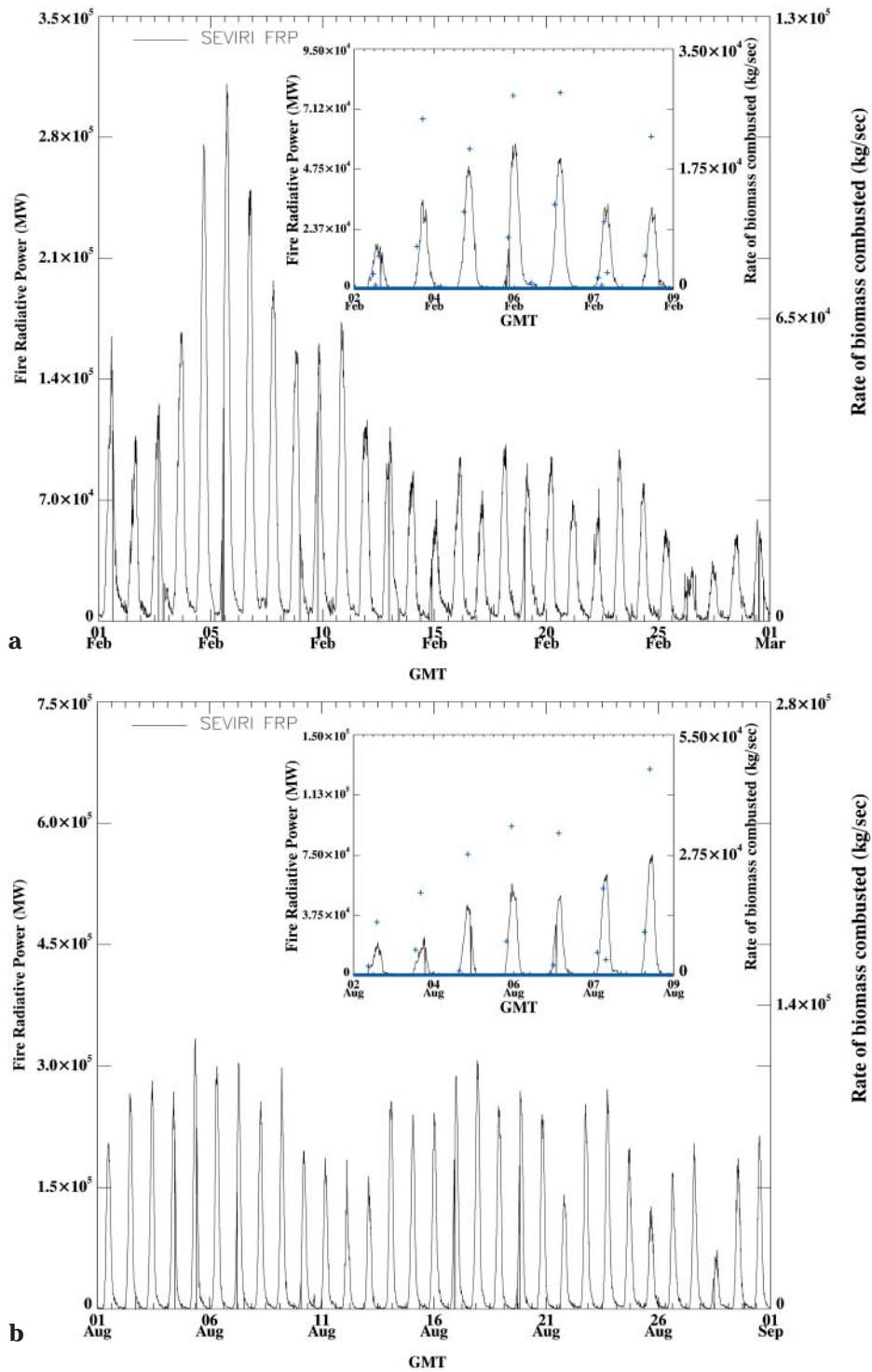
Fig. 1. (a) Spinning Enhanced Visible and Infrared Imager (SEVIRI) fire radiative power (FRP) temporal dynamics over Northern Hemisphere Africa in February 2004. The inset illustrates SEVIRI and Moderate Resolution Imaging Spectroradiometer (MODIS) FRP temporal trajectories over a 10^\circ \times 10^\circ region centered at 5^\circ/15^\circ (latitude/longitude). (b) SEVIRI FRP temporal dynamics over Southern Hemisphere Africa in August 2004. The inset illustrates SEVIRI and MODIS FRP temporal trajectories over a 10^\circ \times 10^\circ region centered at -15^\circ/30^\circ (latitude/longitude). Blue crosses in insets are MODIS FRP data.
