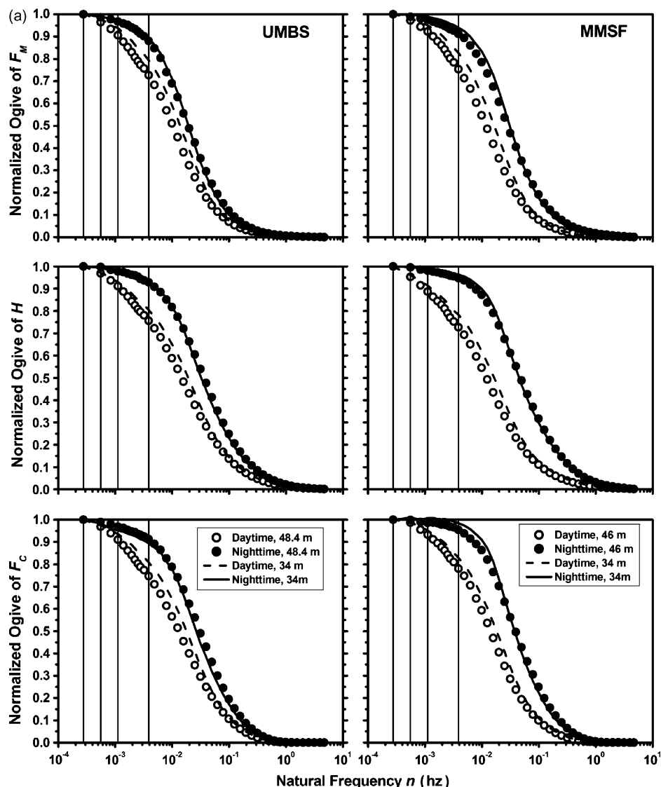
Fig. 6 – (a) Ensemble averages of normalized ogives for momentum, sensible heat and \text{CO}_2 in the upwind directions during the growing season in 2001. The four thin vertical lines in each panel, from left to right, correspond to time periods of 60, 30, 15 and 5 min, respectively. ROT-3 and 1 h averaging time are used with hourly records of 10 Hz raw data. The numbers of ogives are 381 (daytime, 10:00–16:00 LST) and 133 (nighttime, 22:00–04:00 LST) at UMBS, and 356 (daytime) and 203 (nighttime) at MMSF. (b) Effects of averaging time period and sampling frequency on ensemble averages of vertical fluxes of momentum, sensible heat and \text{CO}_2 normalized by fluxes calculated with 1 h averaging time period in the upwind directions during the growing season in 2001. ROT-3 is used with hourly records of 10 Hz data. The numbers of hourly fluxes are 355 (daytime) and 85 (nighttime) at UMBS, and 321 (daytime) and 188 (nighttime) at MMSF.
