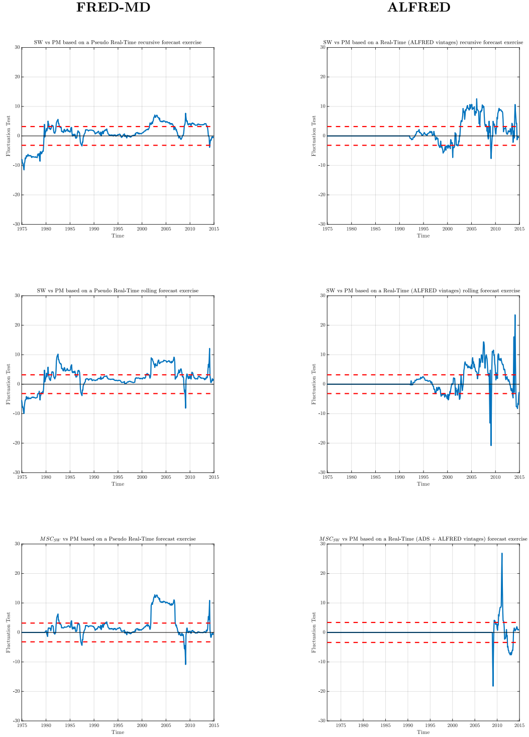
Figure 3: GR test: SW vs PM benchmark
